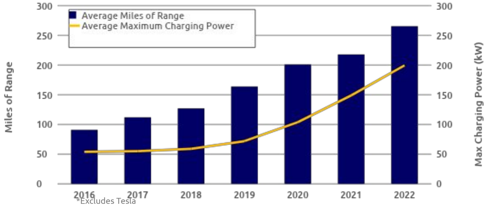
Average Miles of Range and Max Charging Power by EV Model Year*
